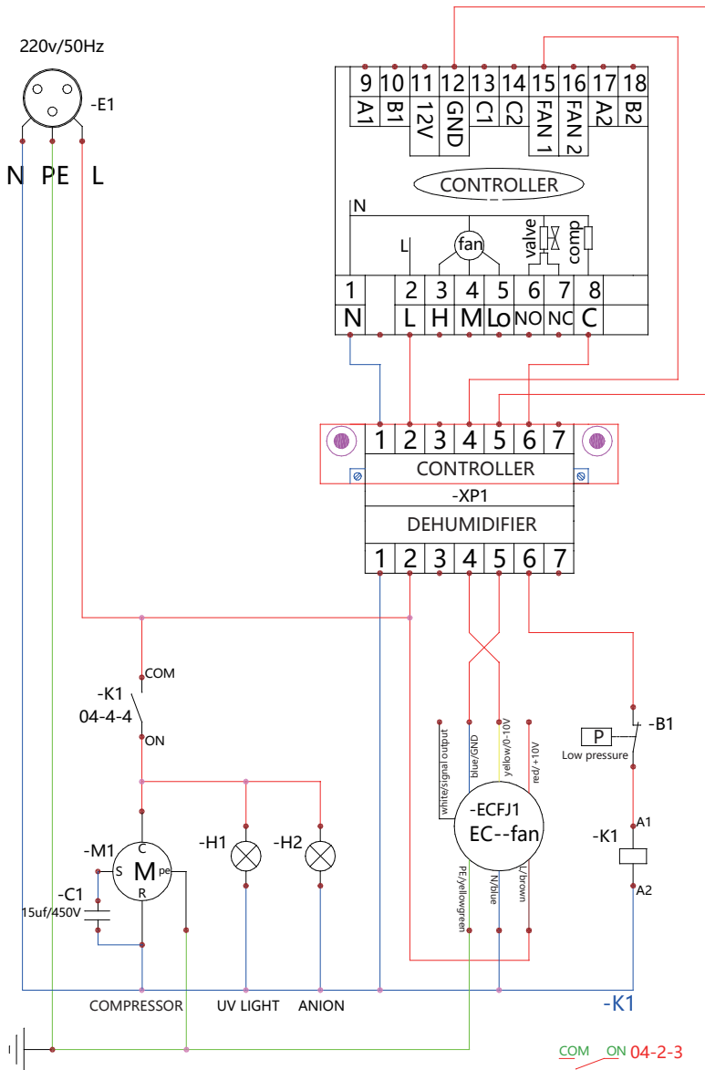
FD-S40/60L-DEHUMIDIFIER WIRING DIAGRAM
