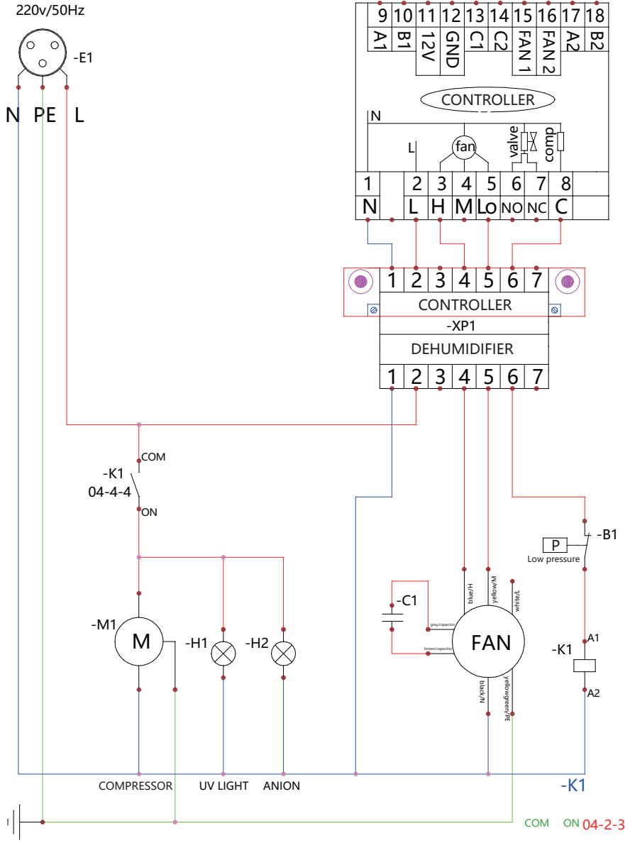
FD-S28L-DEHUMIDIFIER WIRING DIAGRAM
