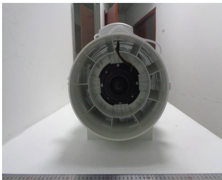
Figure 4 (External view –4)
