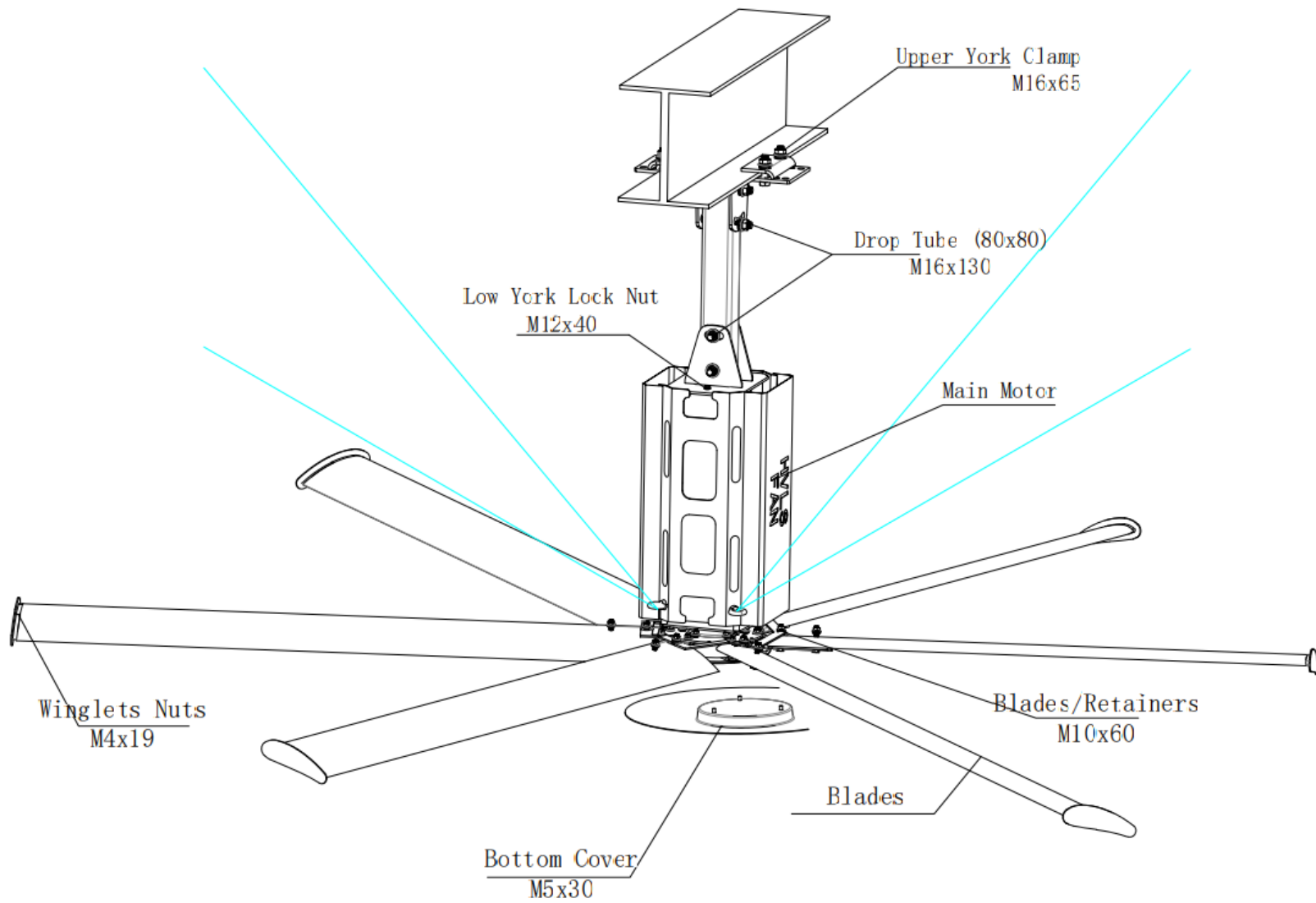
Gearmotor -1.5KW HVLS fan Parts Chart
